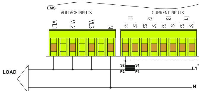
Single-Phase, 2-Wires Configuration
